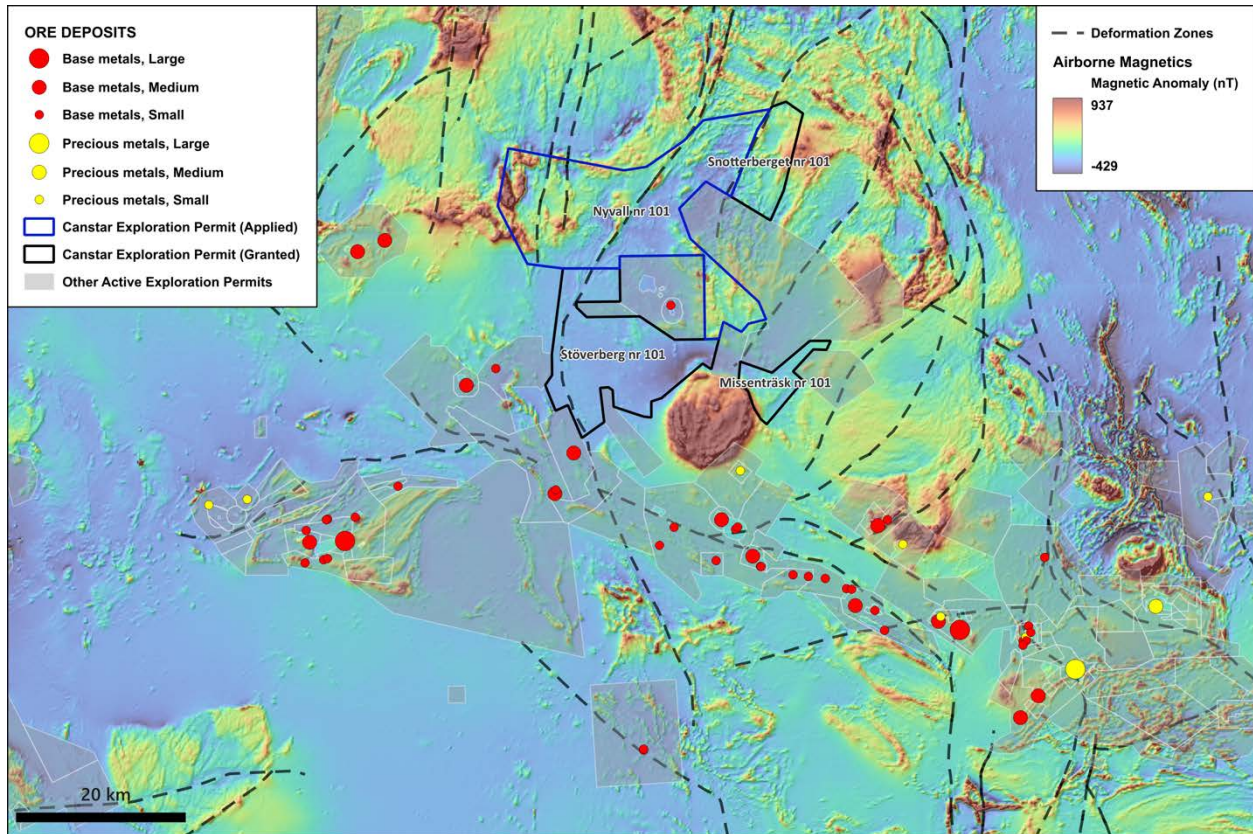
Figure 2 – Airborne magnetic image and structural framework of the Skellefte belt
